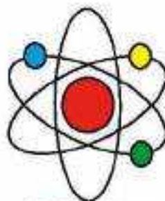
Nuclear atom
