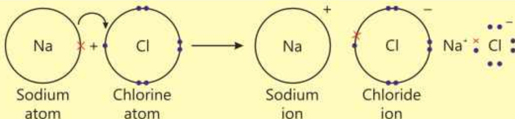
Fig (3.2): Transference of Electron from Sodium to Chlorine Atom
