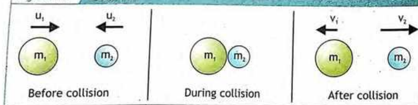
Figure 3.7 Collision
