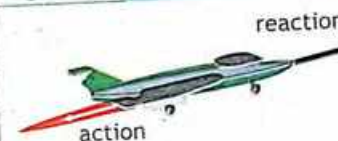
Figure 3.6 Action-Reaction
