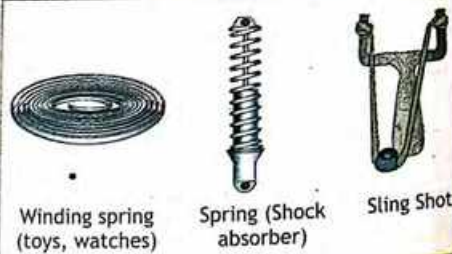
Figure 6.5 Potential Energy
