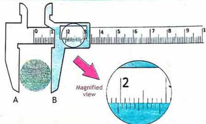
Figure 1.2 Vernier Caliper
