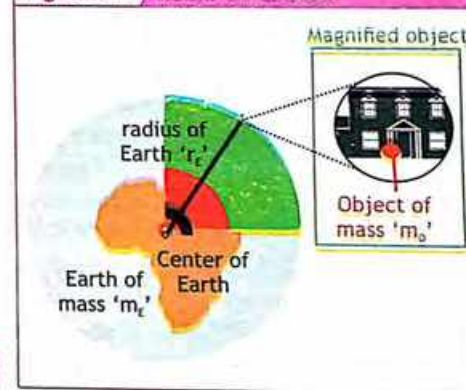
Figure 5.4 MASS OF EARTH
