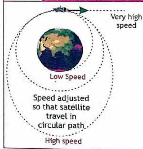
Figure 5.7 SATELLITE MOTION
