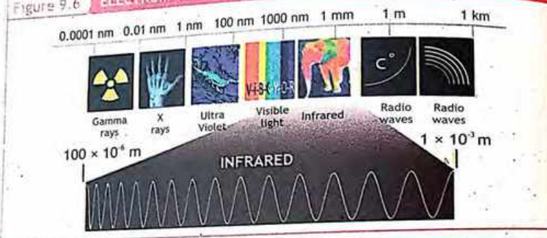
Figure 9.6 ELECTROMAGNETIC SPECTRUM
