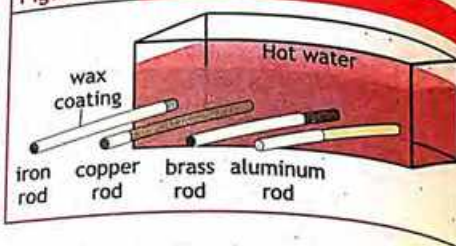
Figure 9.3 CONDUCTION
