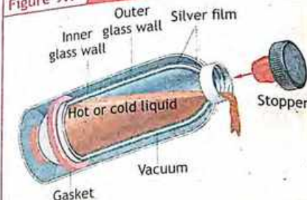
Figure 9.7 THERMOS FLASK
