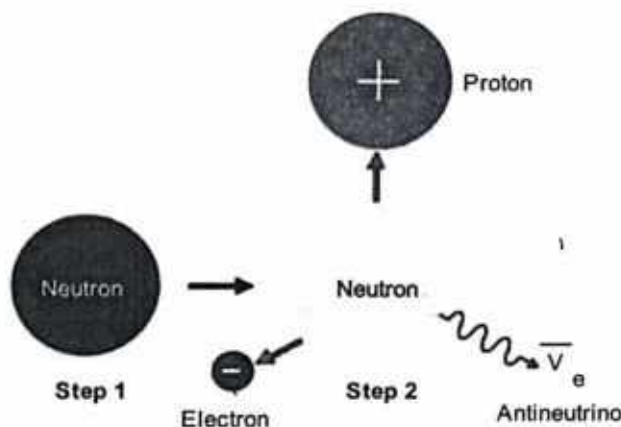
Fig. 9.9: Weak nuclear force (decay of neutron)
