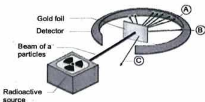
Fig. 4.4: Rutherford's Experiments
