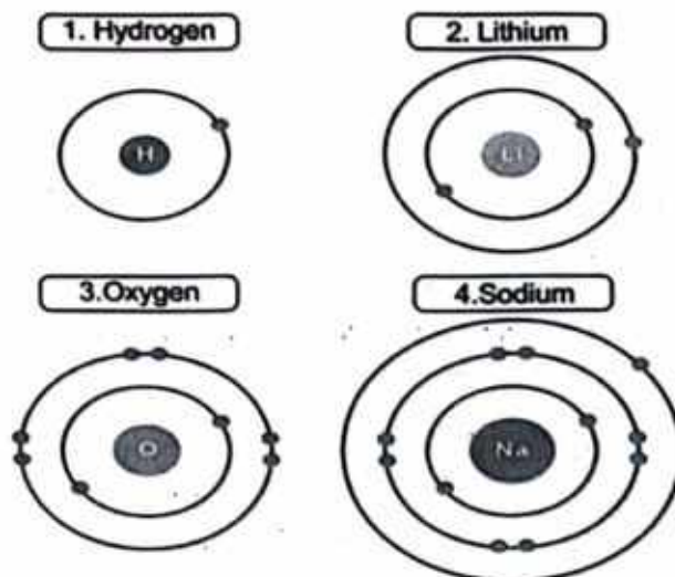
Fig. 4.6: Examples of Bohr's Atomic Model
