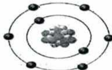
Oxygen-18
