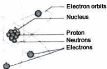
Fig. 4.5: Rutherford Atomic Model
