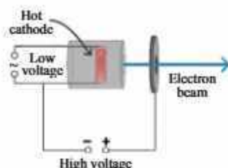
Fig: 17.13. An electron gun
