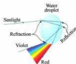
Fig: 12.3. The dispersion by a water droplet
