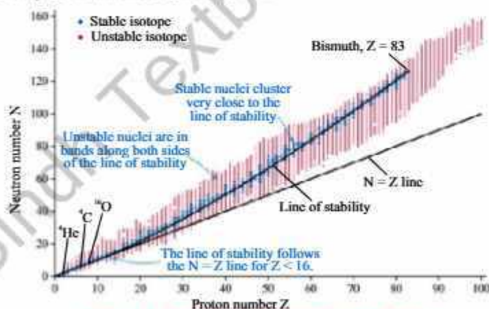
Fig: 20.1. Nuclear stability curve of all isotope
