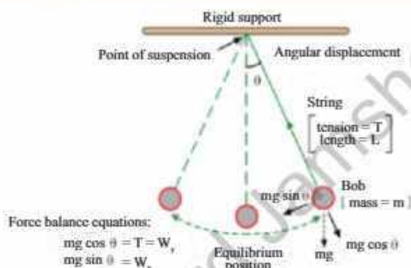
Fig: 10.19. Forces acting on the bob in simple pendulum
