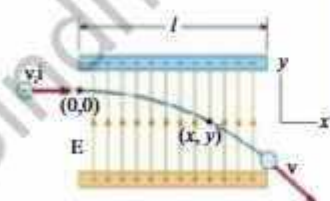
Fig: 17.14. Deflection of electron passing through uniform electric field
