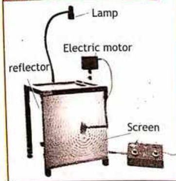
Figure 10.14 - Ripple Tank
