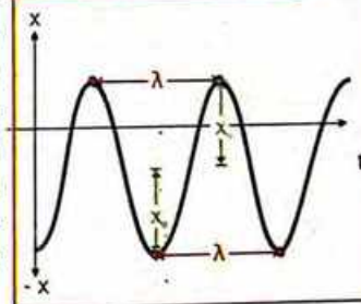
Figure 10.12 - Wavelength
