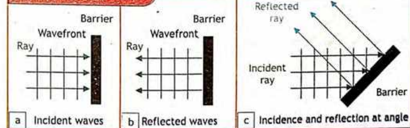
Figure 10.18 - Reflection
