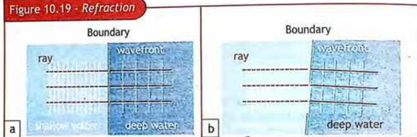
Figure 10.19 - Refraction
