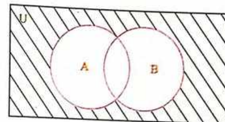
(A \cup B)' (Fig. 1)
