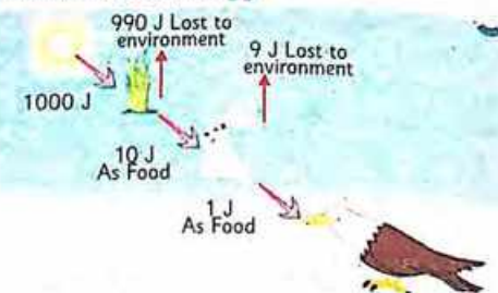
Fig.16.5 Flow of energy in an ecosystem
