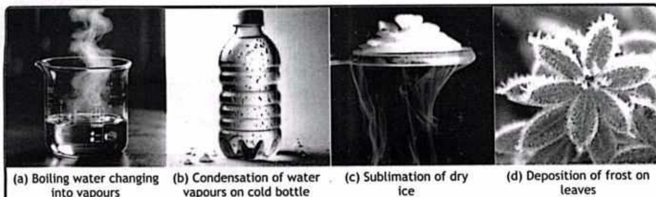
FIGURE 11.3 Changing states of matter
