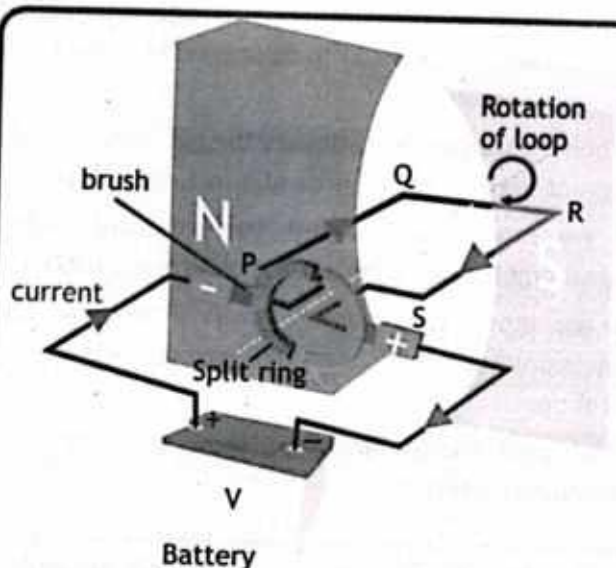
FIGURE 19.13 Electric motor
