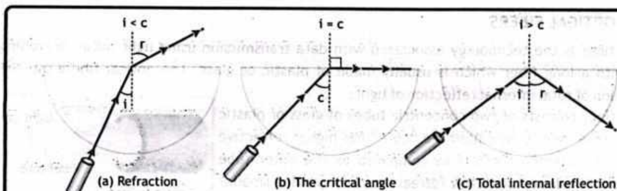
FIGURE 14.7 Experiment for total internal reflection
