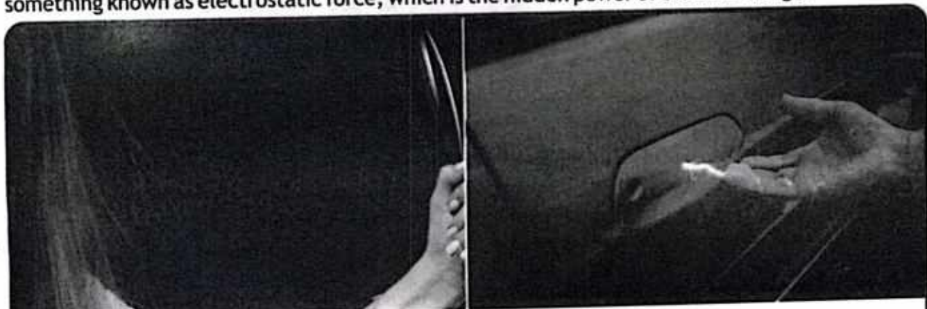
FIGURE 15.1 Electrostatic phenomena
