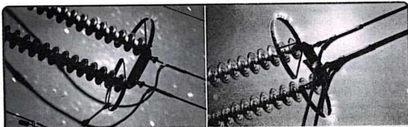
FIGURE 15.21 Corona discharge
