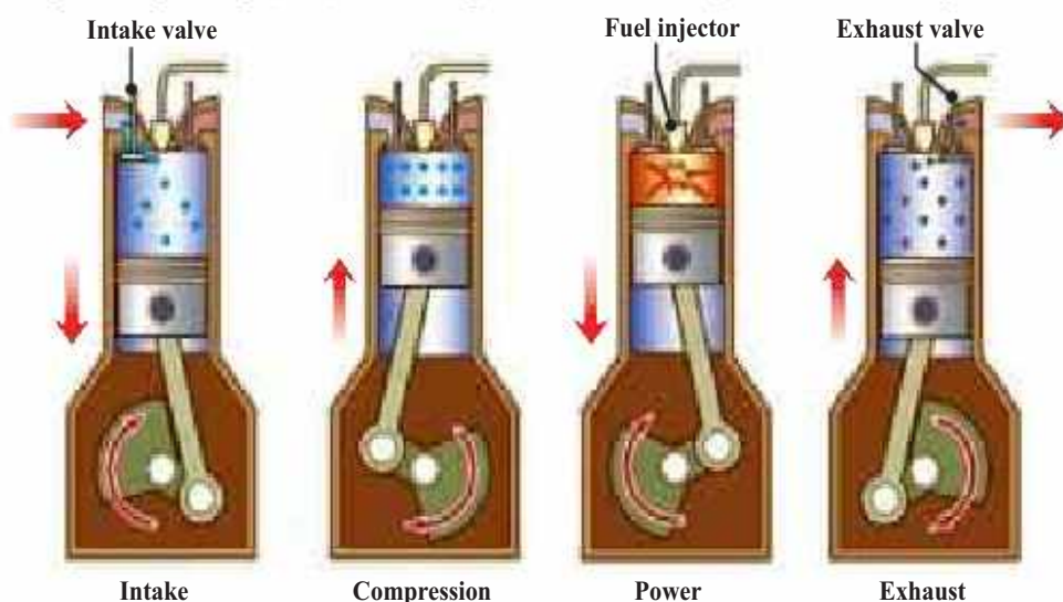
Figure 17.4 Petrol Engine
