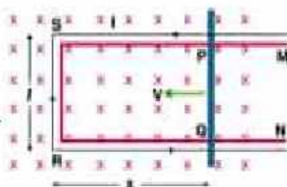
Figure 19.11 Motional emf
