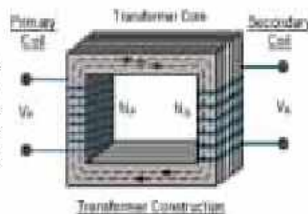
Figure 19.9 Transformer:
