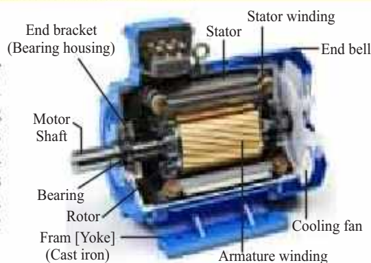
Figure 19.14 AC motor
