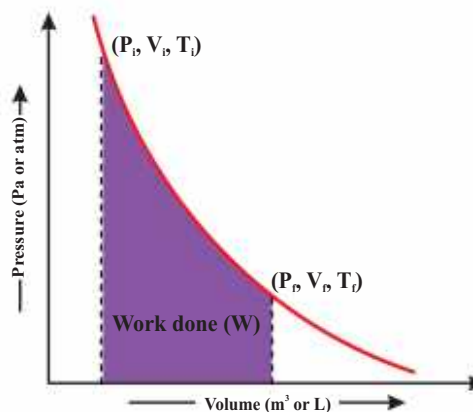
Figure 16.11 graph for adiabatic Compression
