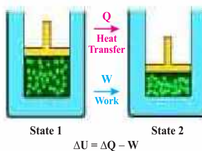
Figure 16.6 states of system
