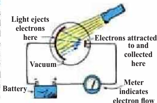
Figure 25.4 Photoelectric Effect
