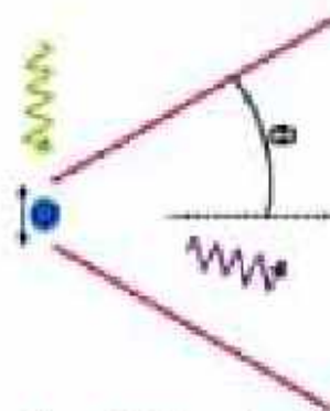
Figure 25.16 Uncertainty Principle
