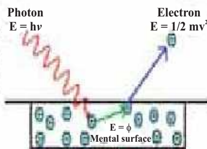
Figure 25.6 photo-electric effect
