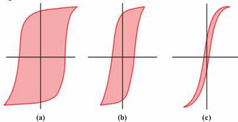
Hysteresis Loops
