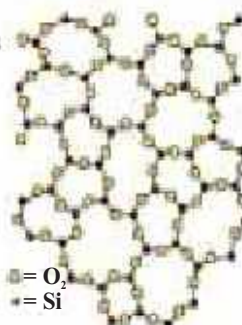
Figure 21.1 structures of crystalline, glassy, amorphous and polymeric solids
