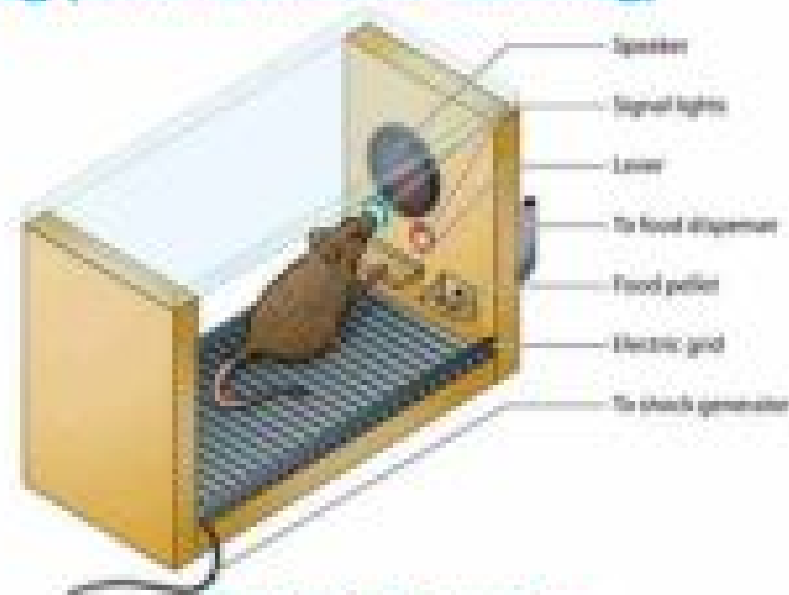
Fig 19.10 Skinner Box
