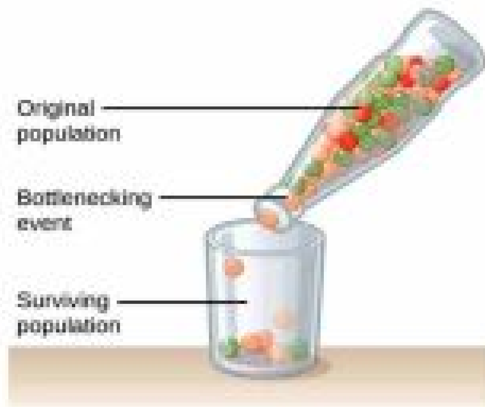
Fig. 24.12 Bottle-neck Effect
