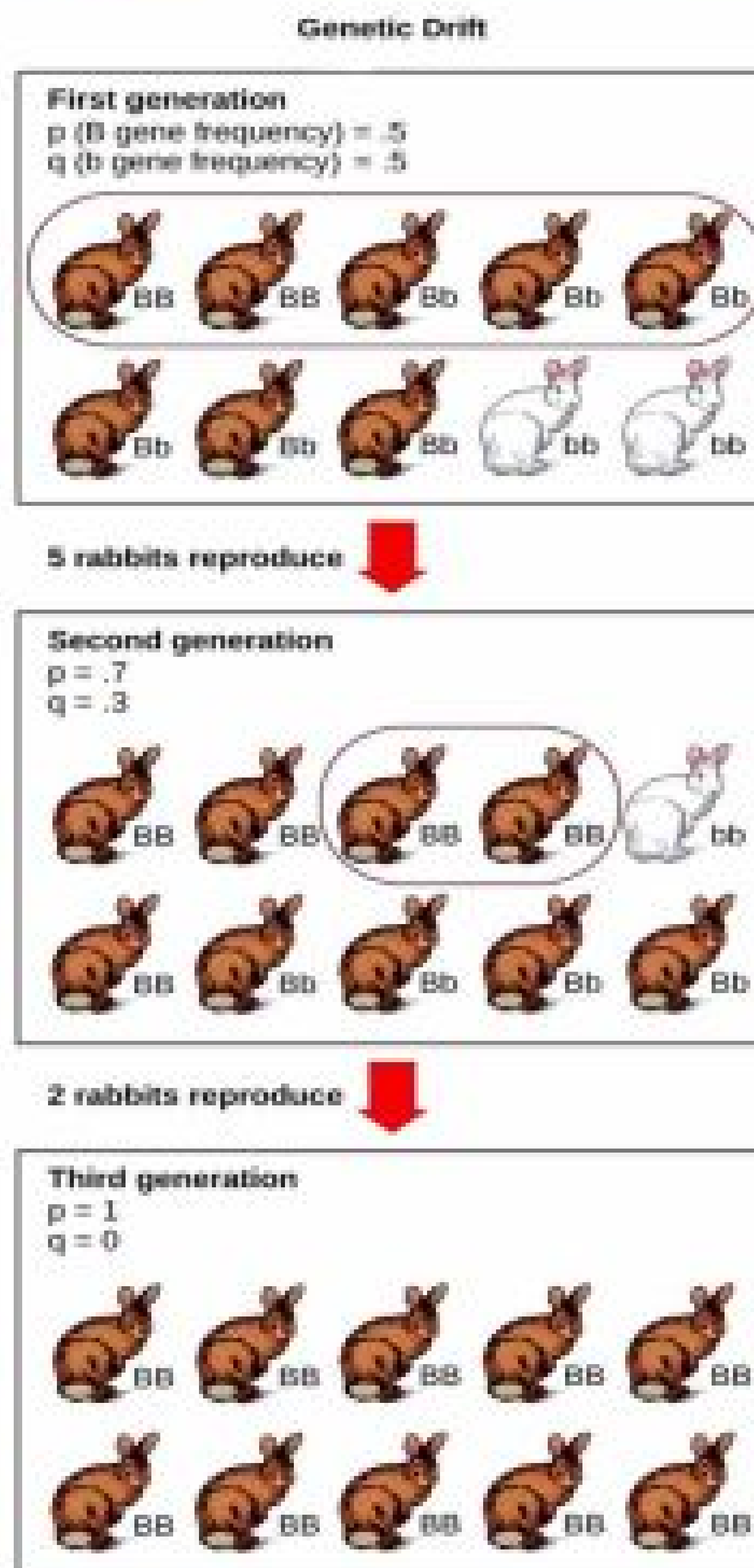
Fig. 24.10 Genetic drift
