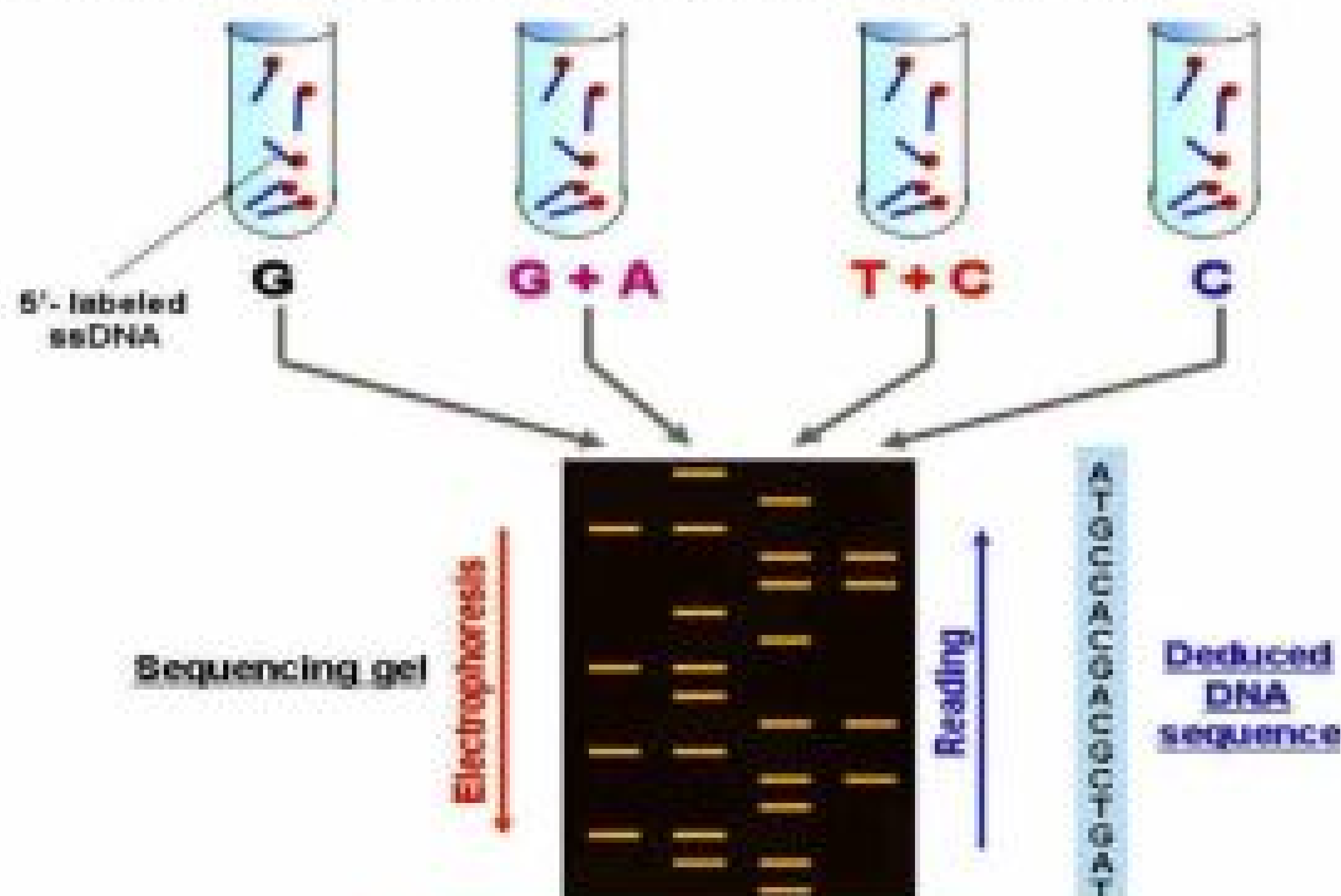
Fig.26.7 Maxam-Gilbert Method
