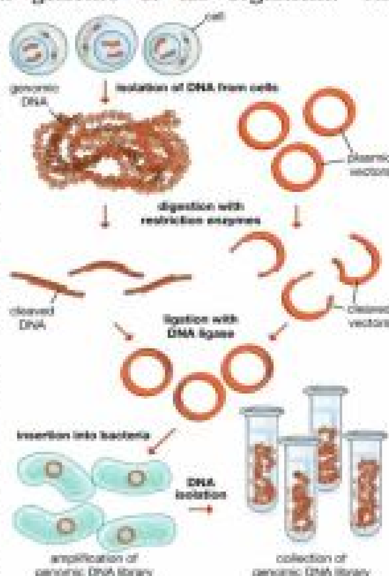
Fig.26.6 Genomic Library
