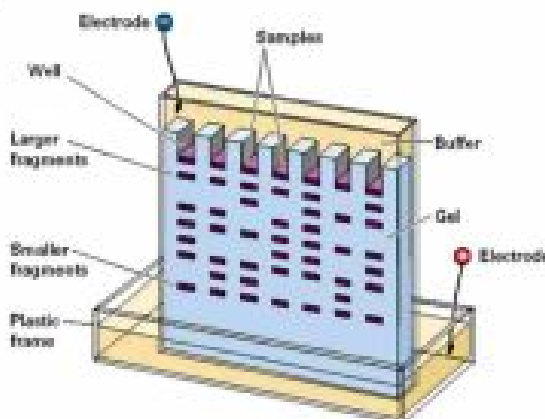
Fig.26.9 Electrophoresis
