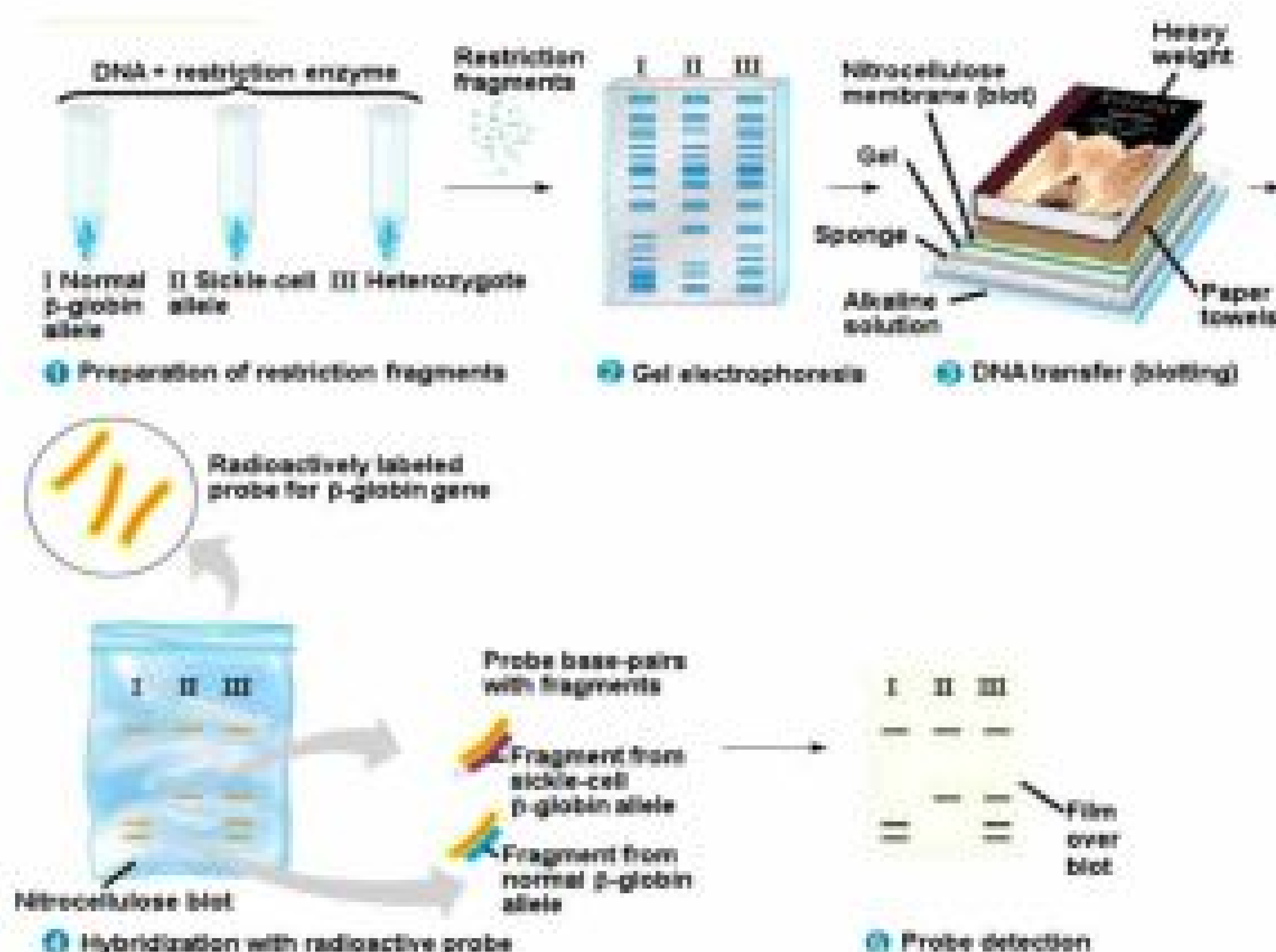
Fig. 26.10 DNA analysis
