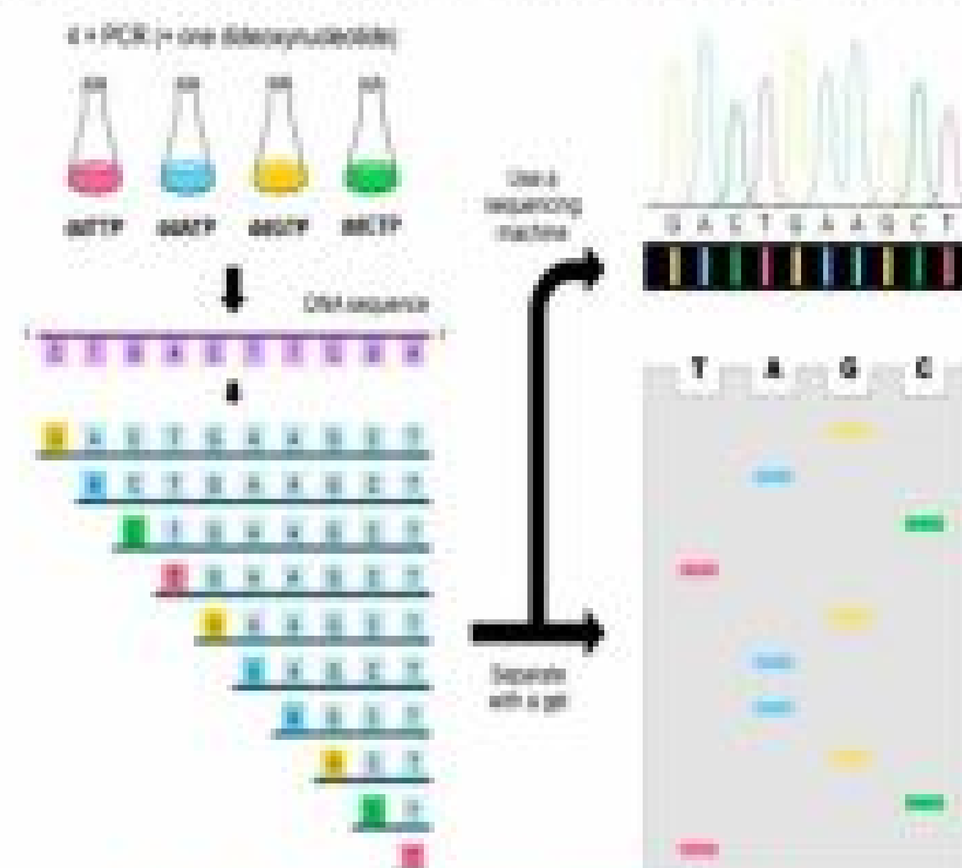
Fig.26.8 Singer-Coulson Method
