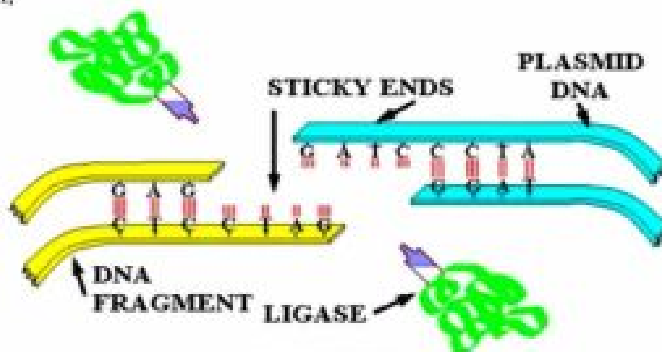
Fig.26.3 DNA ligase
