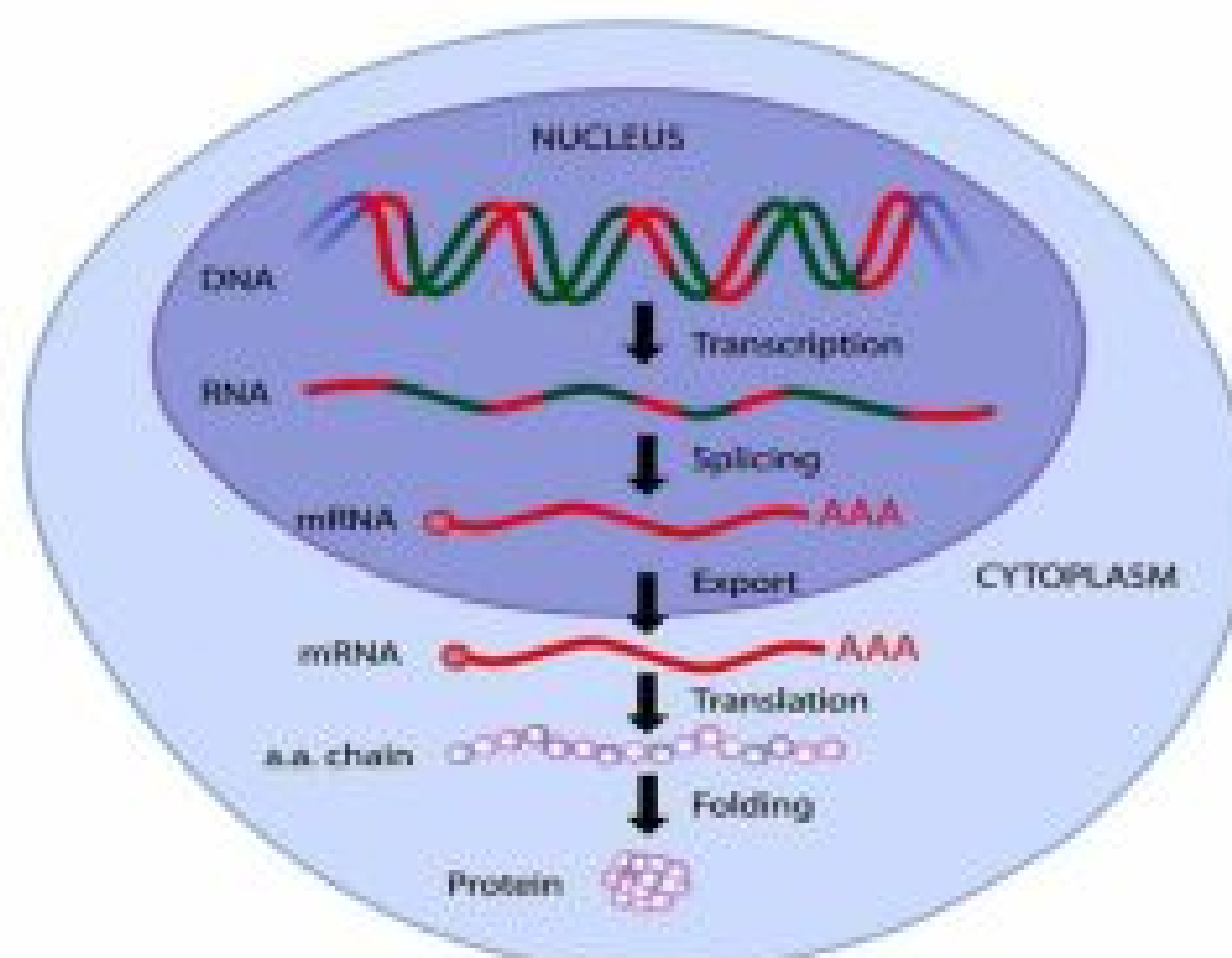
Fig.22.13. Gene expression
