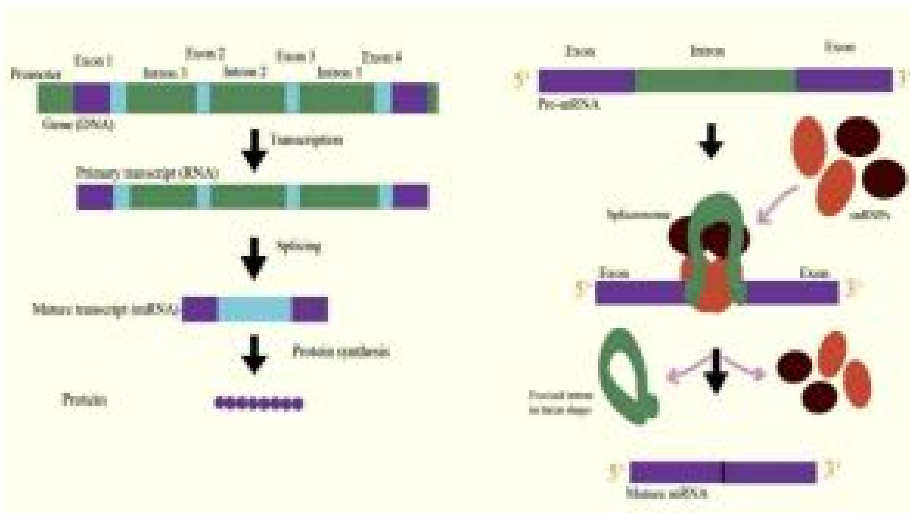
Fig.22.16.RNA splicing
