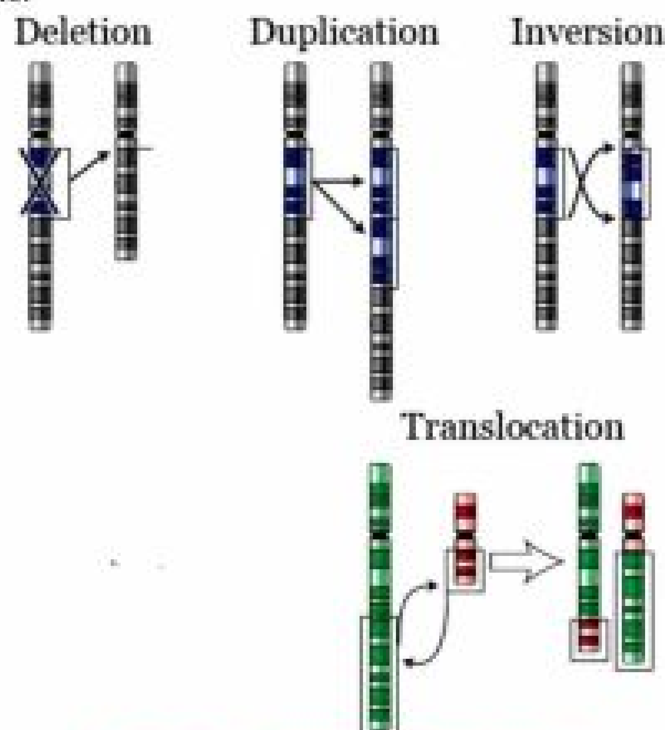
Fig.22.18. Chromosomal Aberration
