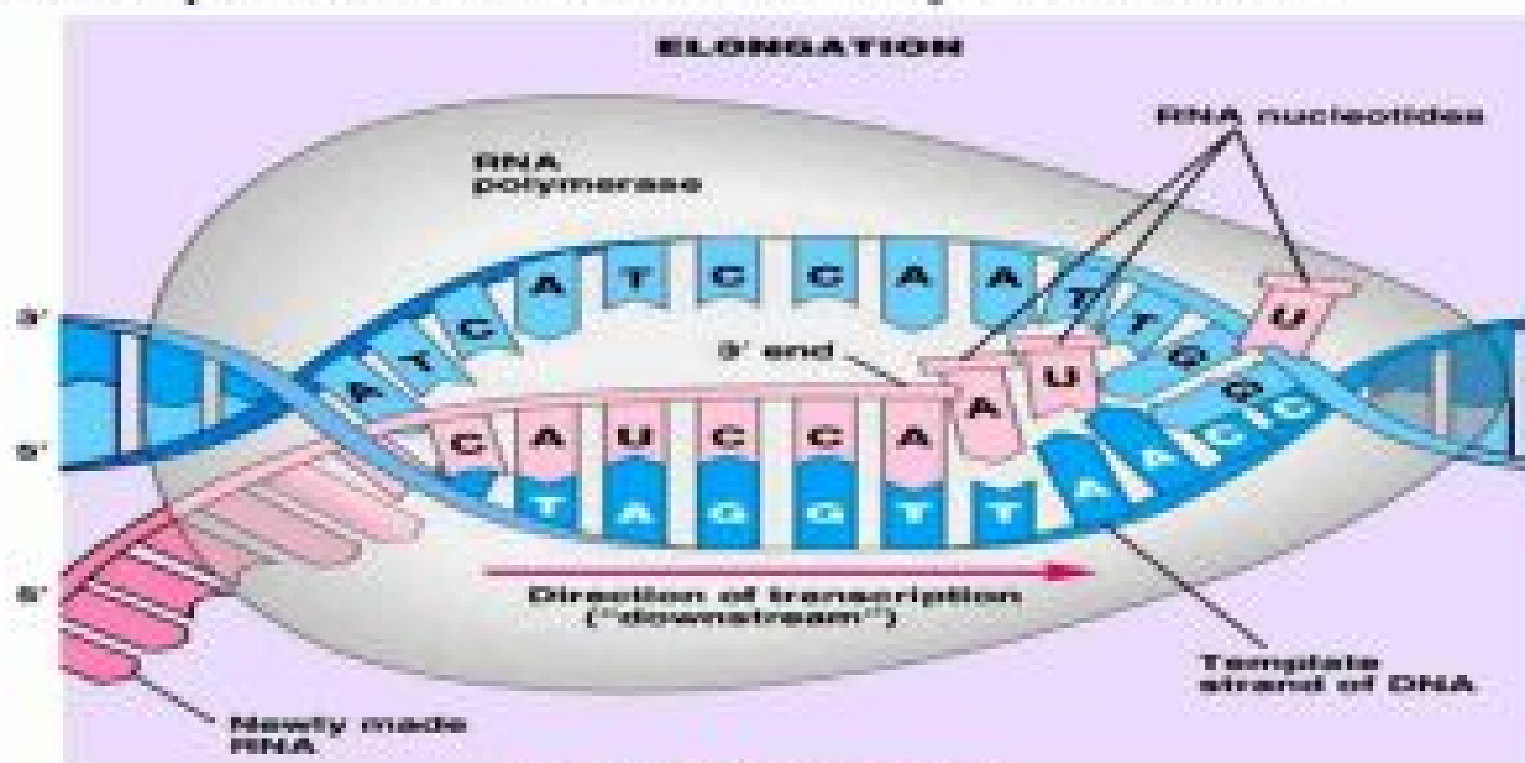
Fig.22.15.Transcription
