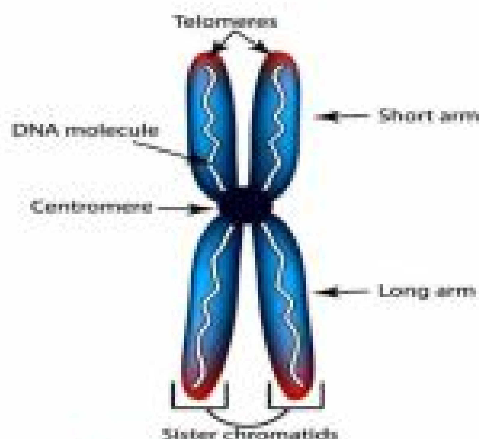
Fig. 22.1 Chromosome
