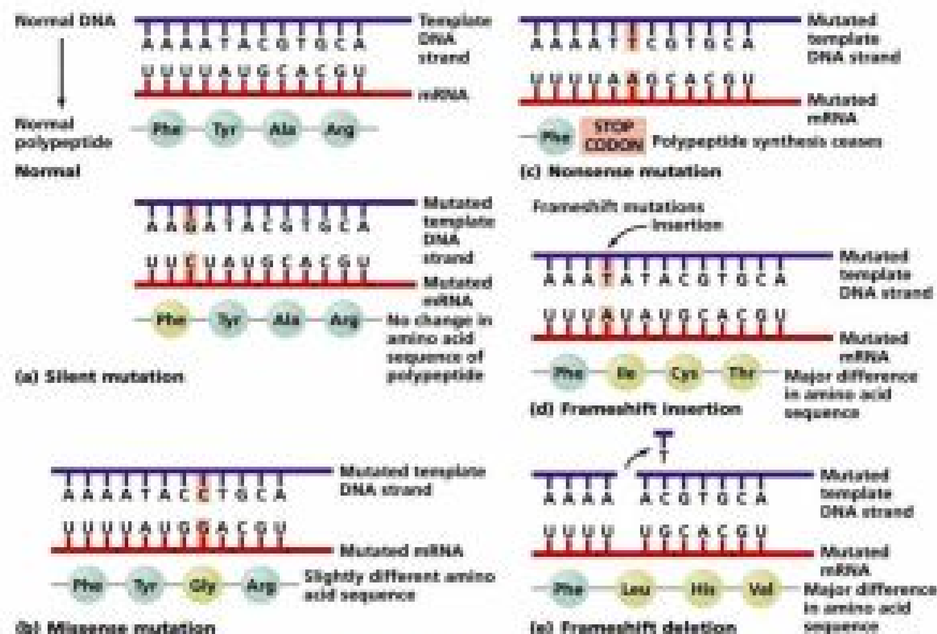
Fig.22.19.Gene mutation
