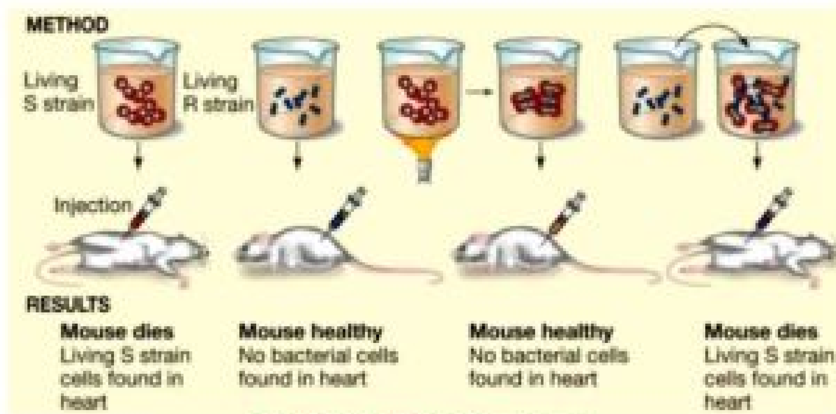
Fig.22.6. Griffith's Experiment
