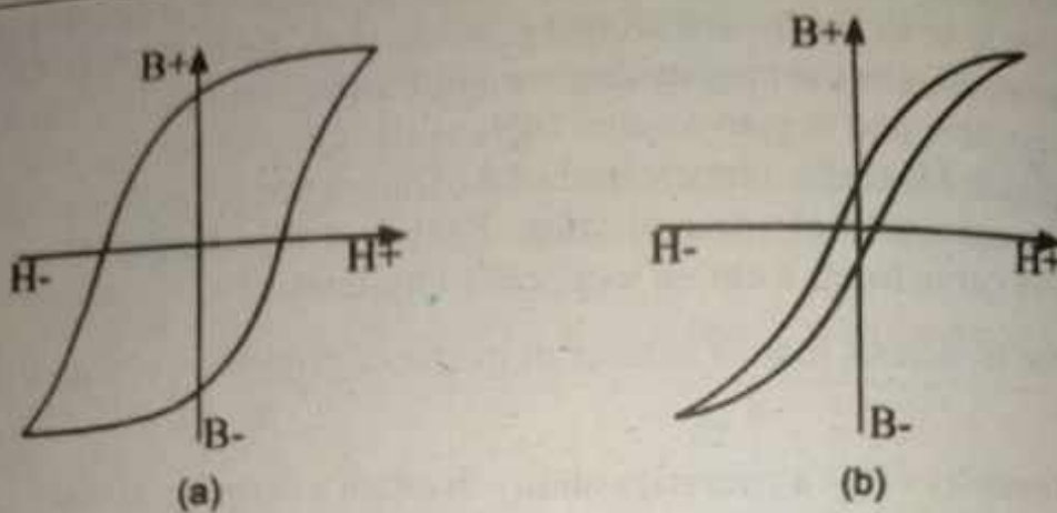
Figure 16.18: (a) the hysteresis loop for hard magnetic material suitable for permanent magnet; (b) the hysteresis loop for soft magnetic material suitable for a transformer core.
