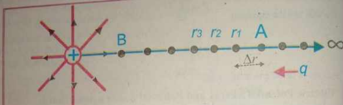
Figure 11.24: work done on a test charge q in moving it towards source charge +Q
