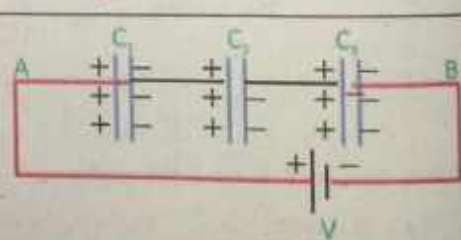
Figure 11.30(a) : series combination of capacitors
