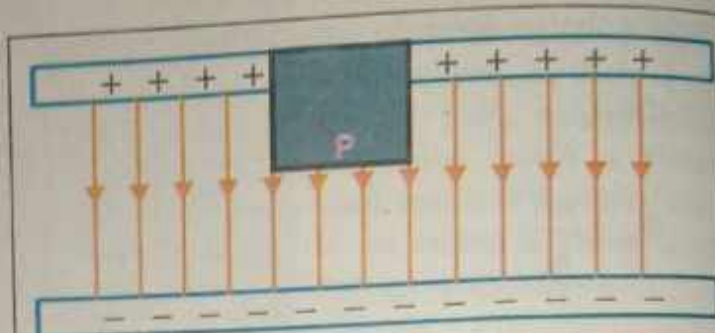
Figure 11.22: Gaussian surface in the form of a box between the plates
