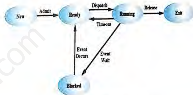
Figure 1.10: Five-State Process Model
