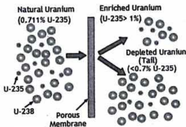
Figure 22.18: Gaseous diffusion uranium enrichment process.
