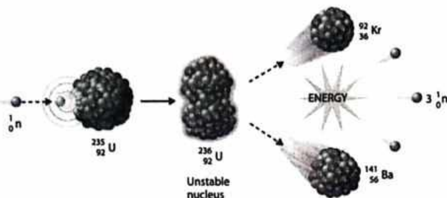
Figure 22.13: Fission reaction.
