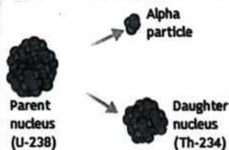
Figure 22.3: Alpha decay of U-238.
