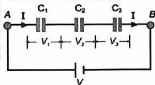
Figure 19.4: Series combination of capacitors.
