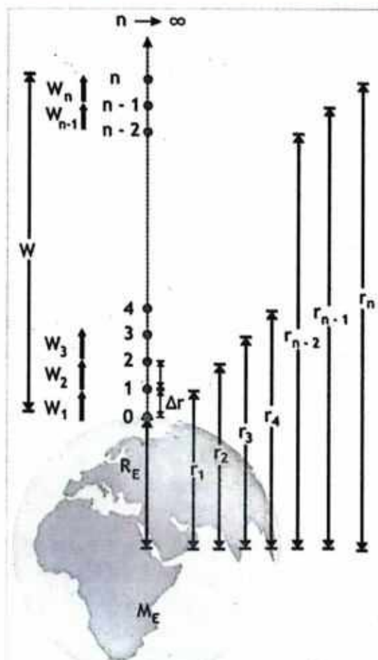
Figure 15.10: Gravitational Potential.
