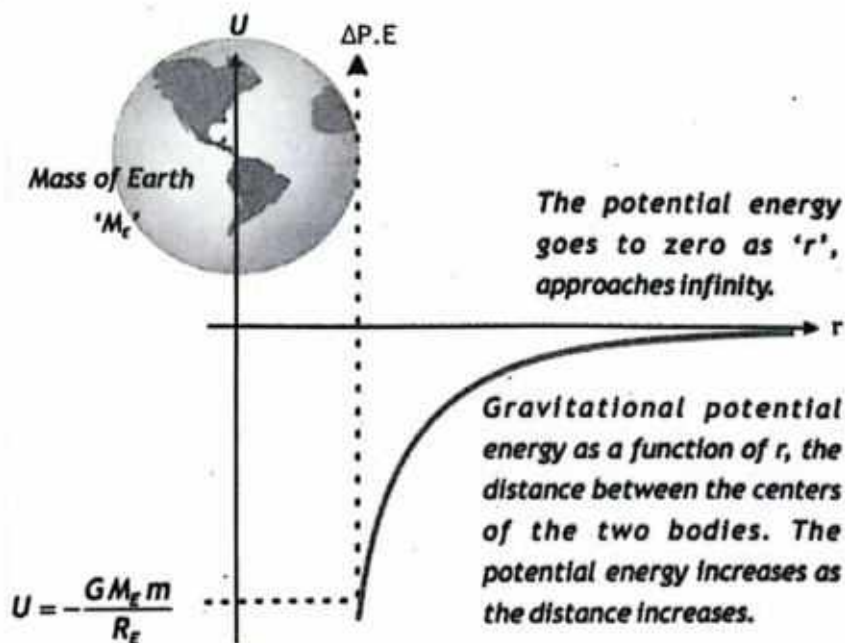
Figure 15.11: Variation of the gravitational field and potential, as a function of the distance from the center.
