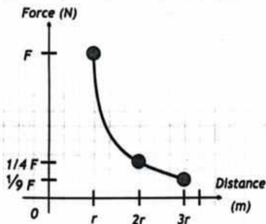
Figure 15.2: Variation of the gravitational force as a function of the distance.
