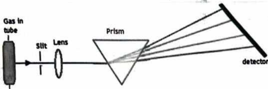
Figure 21.12: Setup for obtaining spectrum.
