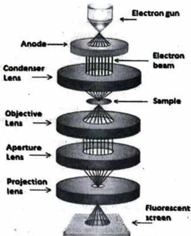
Figure 21.10: Electron microscope.
