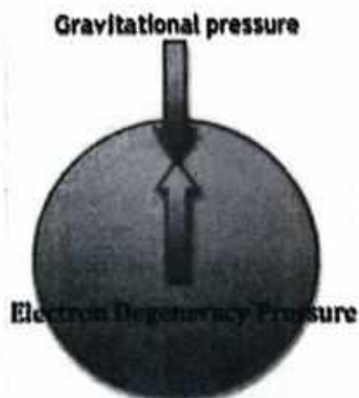
Figure 16.5: Degeneracy pressure.
