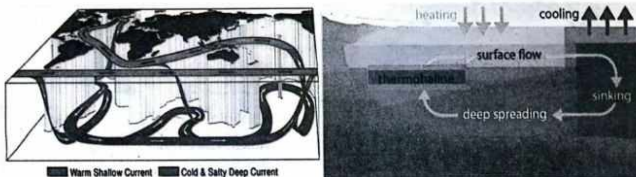
Figure 24.9: Thermohaline circulation.
