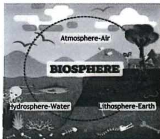
Figure 24.6 (b): Biosphere
