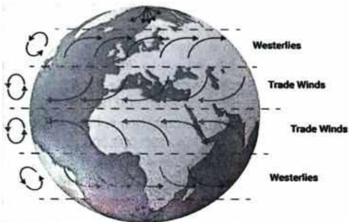
Figure 24.7: Coriolis force.
