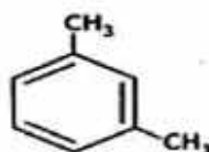
1,3-dimethylbenzene (m-xylene)
