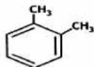
1,2-dimethylbenzene (o-xylene)
