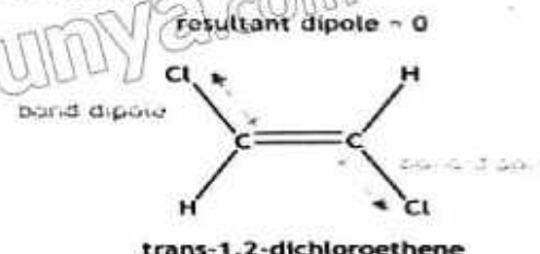
trans-1,2-dichloroethene
