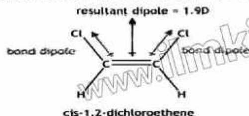
cis-1,2-dichloroethene
