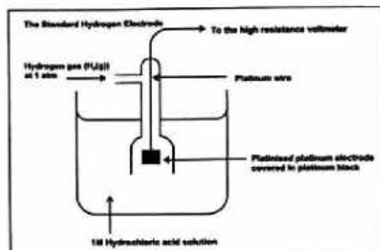
Fig 2.2: Standard Hydrogen Electrode
