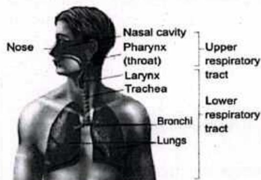
Fig. 3.1: Human respiratory tract
