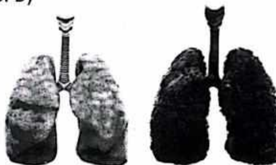
Fig. 3.12: Effects of smoking on lungs
