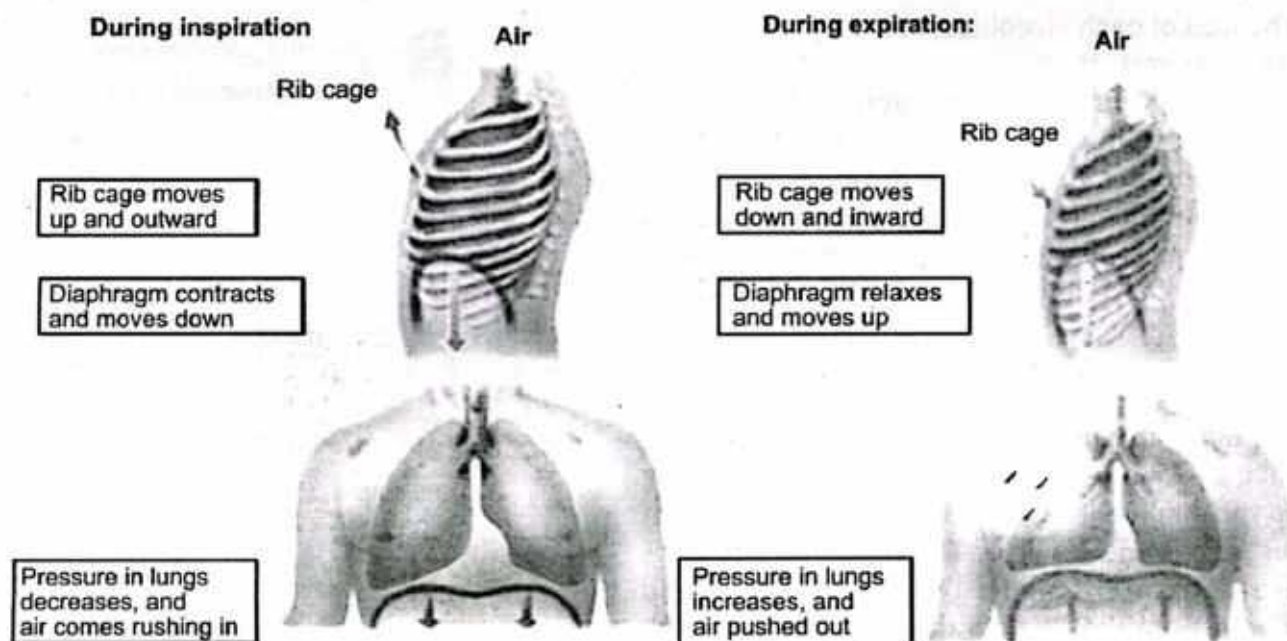
Fig. 3.5: Mechanism of breathing in human
