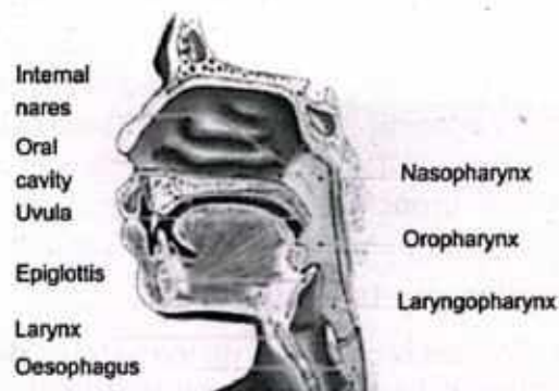
Fig. 3.2: Human respiratory tract
