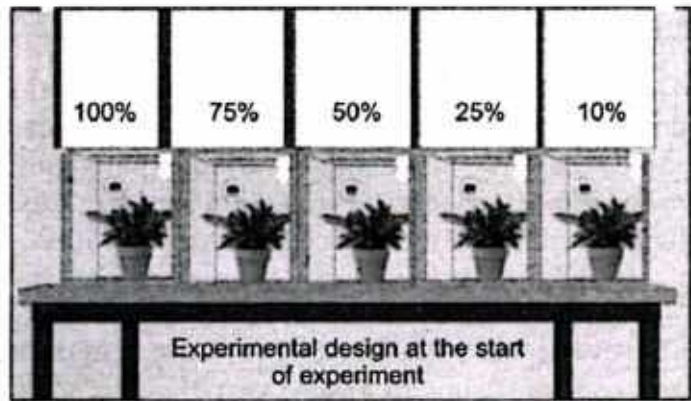
Fig. 11.3: Experimental design to check the effect of light intensity on plant growth
