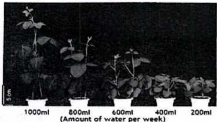
Fig. 11.6: Experimental results showing the effect of amount of water on plant growth
