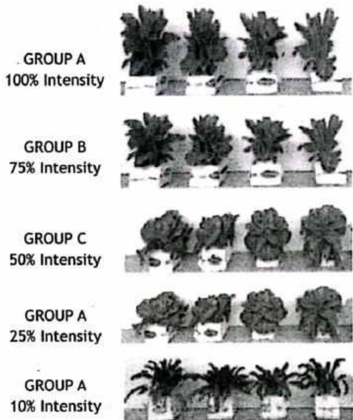
Fig. 11.4: Experimental results showing the effect of light intensity on plant growth
