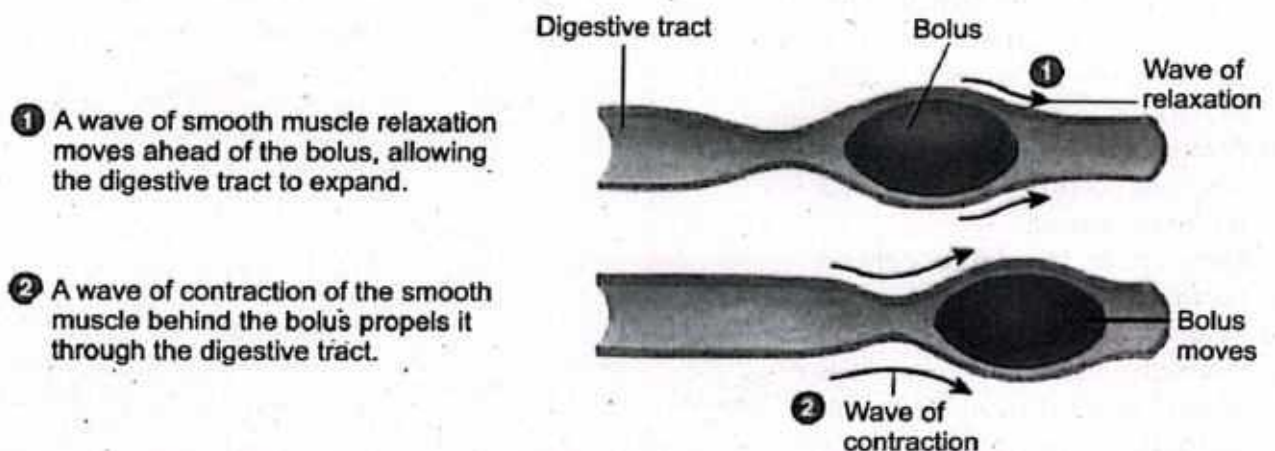
Fig. 1.6: Peristalsis
