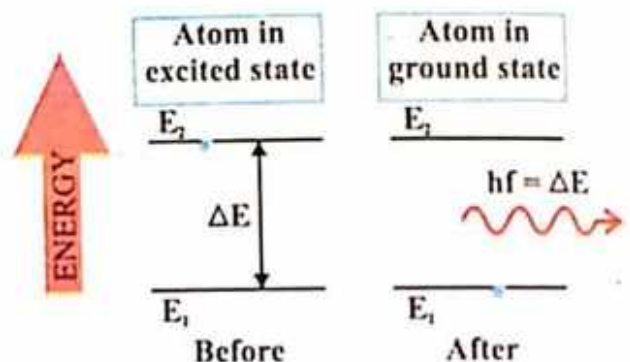
Fig.19.9. the process of spontaneous emission of photon due to the transition of electron from the excited state to the ground state.
