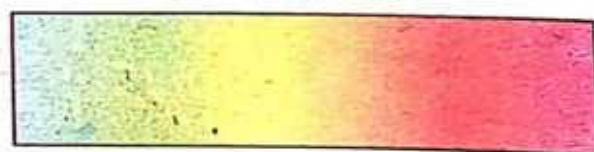
(c) Continuous Spectrum
