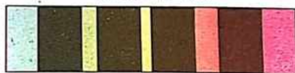
(b) Band Spectrum
