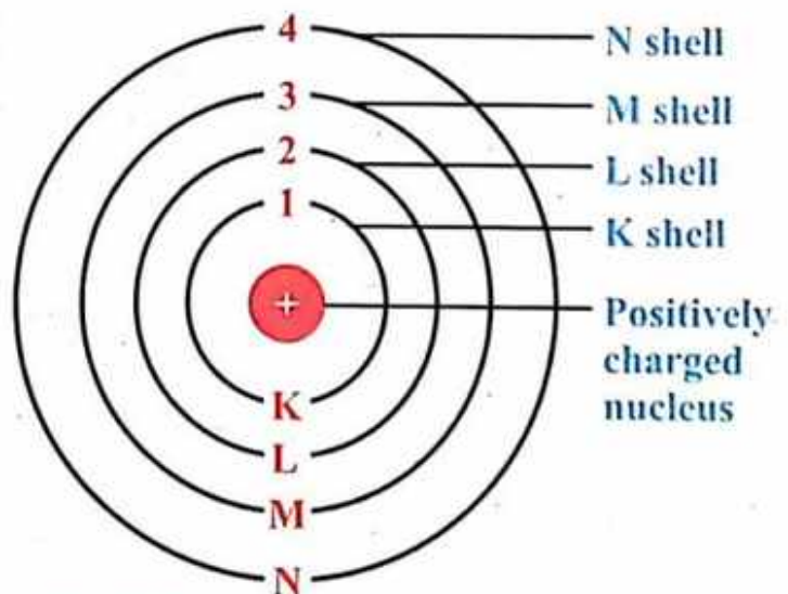
Fig.19.7(a). An isolated atom possessed a number of concentric shells.
