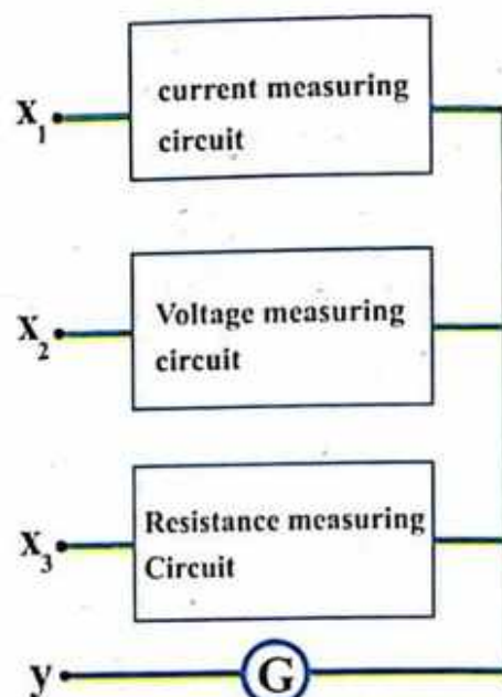
Fig.13.29 A network of an avometer.
