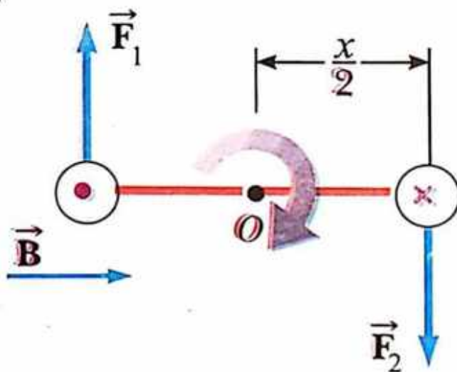
Fig.13.21(a) A magnetic field parallel to the plane of the loop, where F_1 and F_2 act perpendicularly on moment arm x/2 and produce maximum torque.
