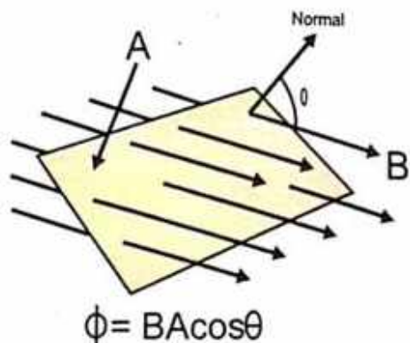
Fig.13.7 The magnetic field lines passing through area.
