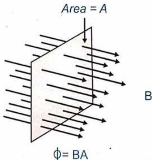
Fig.13.8 Area held perpendicular and angle \theta between B and A is 0^\circ .
