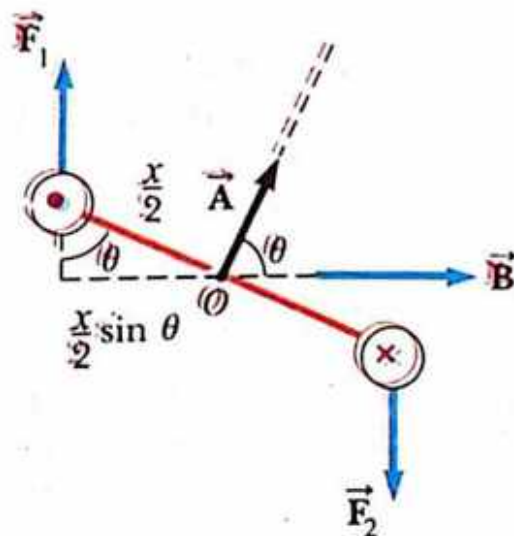
Fig.13.21(b) There is some angle between field \vec{B} and area \vec{A} of the loop and torque is due to the forces F_1 and F_2 and vertical components of moment arm (x/2 \sin \theta)
