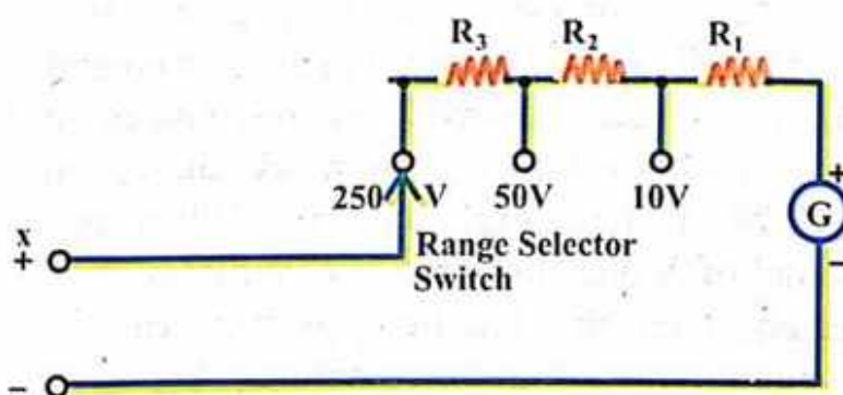
Fig.13.31 A circuit diagram for voltage measuring of an avometer.
