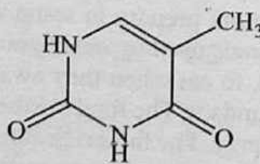
Thymine
