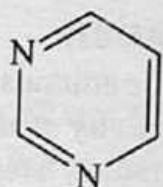
Pyrimidine
