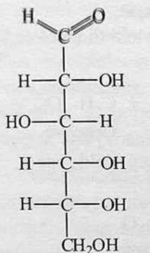
Open chain structure
