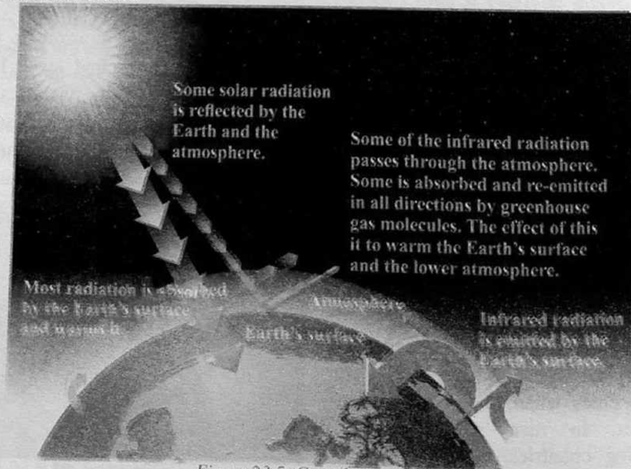
Figure 23.5: Greenhouse Effect
