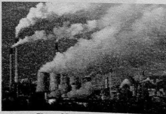
Figure 23.4: Industrial Smog
