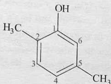
2,5-Dimethylphenol
