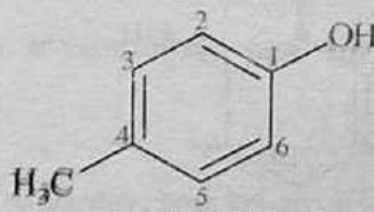
4-Methylphenol ( p -Cresol)
