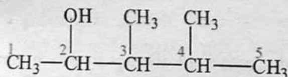
3,4-dimethyl-2-pentanol
