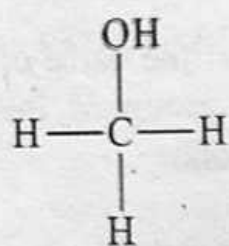
Methanol
