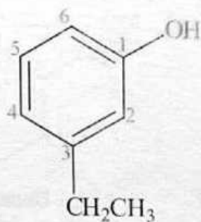
3-Ethylphenol ( m -Ethylphenol)
