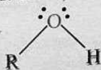
Alcohol
