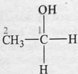
Ethanol
