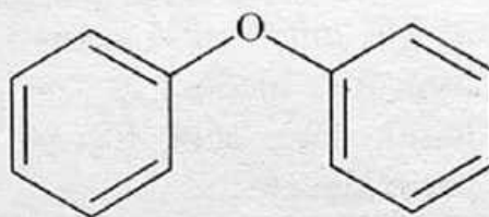
Diphenyl ether
