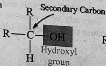
Secondary alcohol
