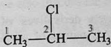
2-Chloropropane
