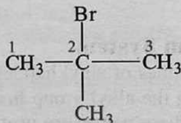
2-Bromo-2-methylpropane
