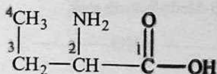
2-Aminobutanoic acid
