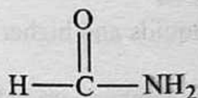
Methanamide (Formamide)
