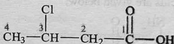
3-Chlorobutanoic acid
