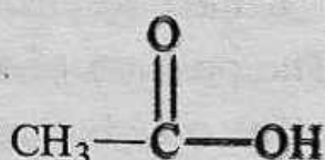
Ethanoic acid
