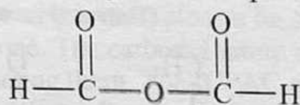
Methanoic anhydride (Formic anhydride)
