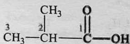
2-Methylpropanoic acid
