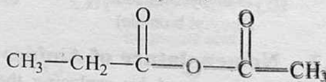
Ethanoicpropanoic anhydride (Acetiopropionic anhydride)
