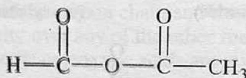
Ethanoicmethanoic anhydride (aceticformic anhydride)
