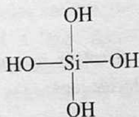
Orthosilicic acid
