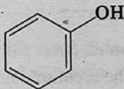
Phenol
