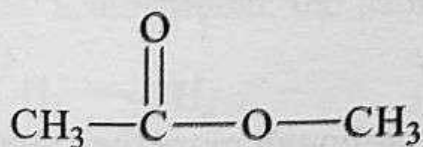
Methyl acetate
