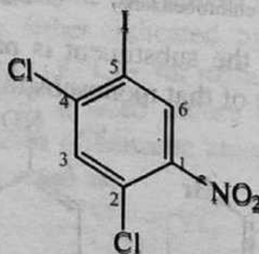
2,4-Dichloro-5-iodonitrobenzene
