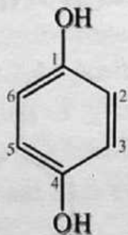
Hydroquinone
