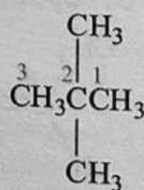
Neopentane
