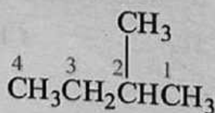
Isopentane
