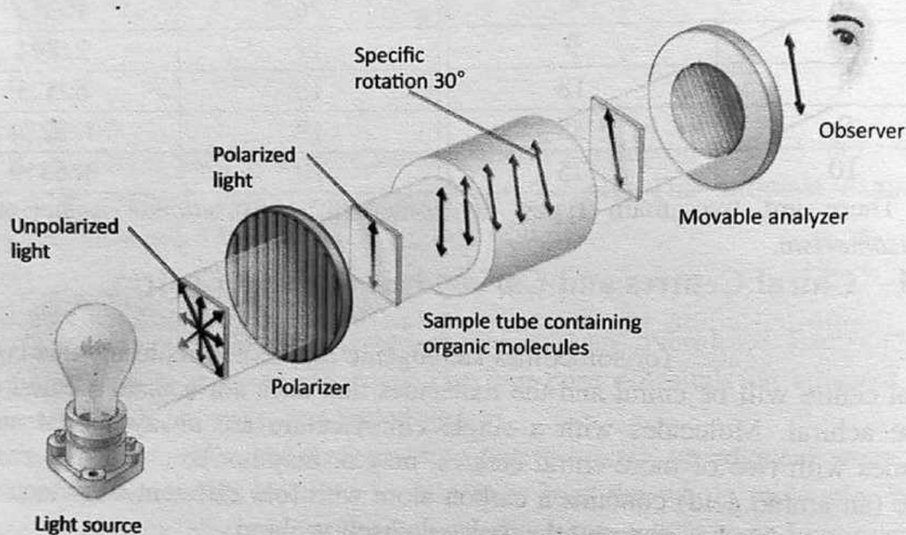
Figure 16.3: Polarimeter
